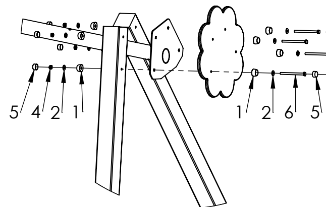
DETAIL B SCALE 1 : 20
